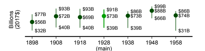
Fig. 3. Cumulative damages due to historical precipitation change. (A) Cumulative observed flood damages (gray) and estimated portion due to historical precipitation change (green) from 1988 to 2017. Error bars show the 95% CI for cumulative damages in 2017 (based on precipitation trends from 1928 to 2017). (B) Impact of historical precipitation change on cumulative flood damages in 2017 using various regression model specifications. From left to right, the models are the regional model (same as A), the regional-seasonal model (Fig. 1D), a regional model with lagged precipitation (SI Appendix, Fig. S2A), a linear model (Fig. 1B), and a quadratic model (Fig. 1B). (C) Sensitivity of cumulative damages from precipitation change to starting year of precipitation trend calculation. All estimates use the same regional regression model used in A.
